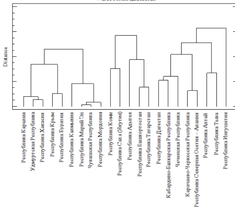
Dendrogram Ward's Method, Euclidean
