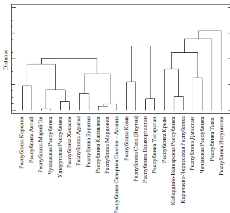
Dendrogram Ward's Method, Euclidean
